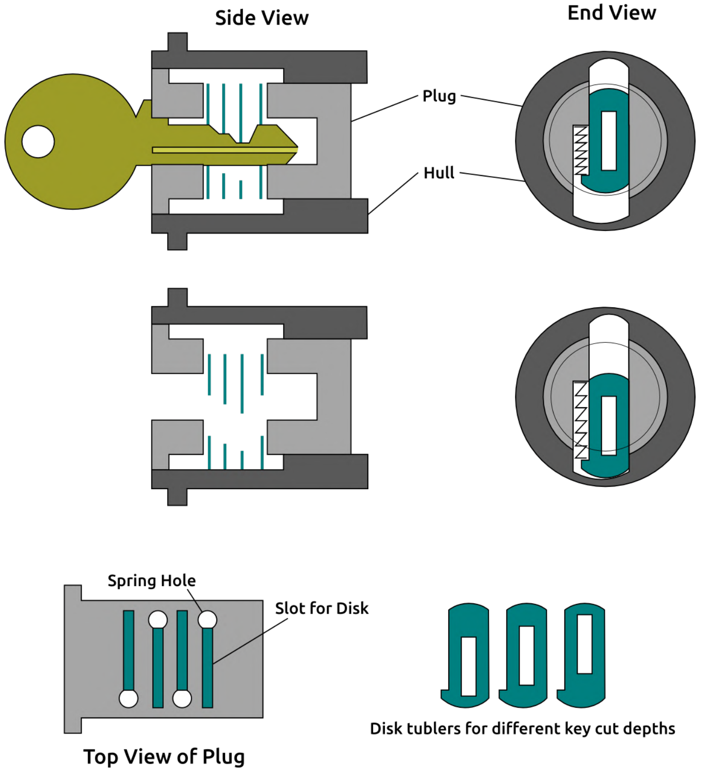
Figure 9.10: Workings of a disk tumbler lock
